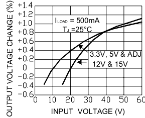
Line Regulation
