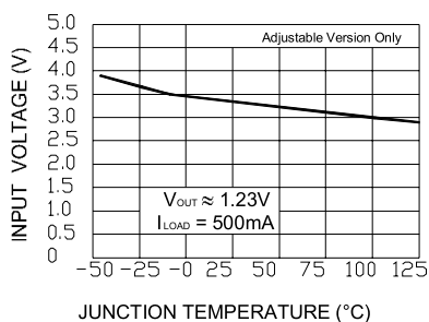
Minimum Operating Voltage
