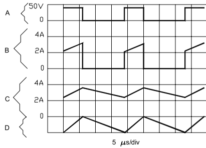
Switching Waveforms
