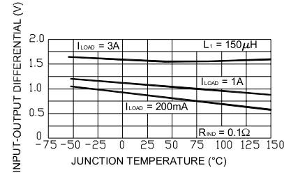
Dropout Voltage
