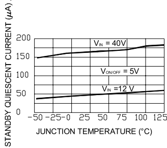
Standby Quiescent Current
